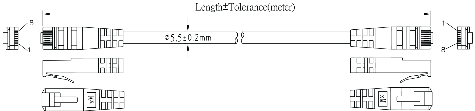
RJ45 8P8C PLUG 50μ
